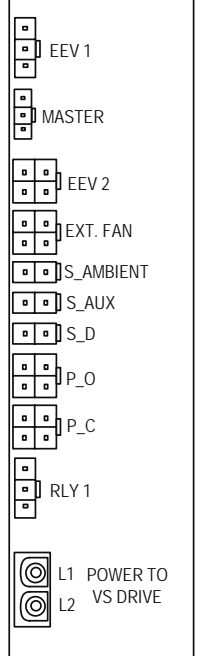
VARIABLE SPEED DRIVE END VIEWS
