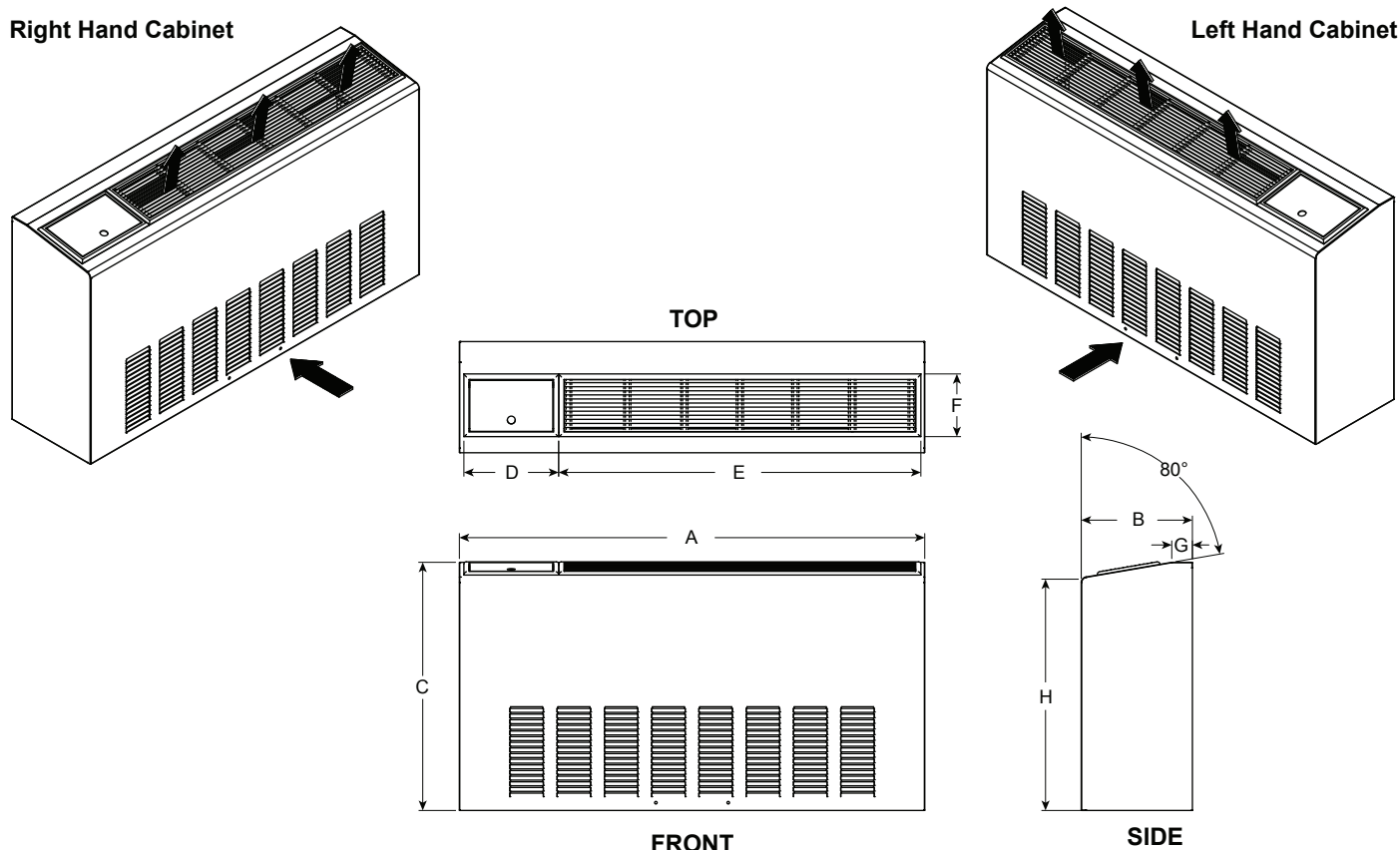
Right return cabinet shown in dimensional views
