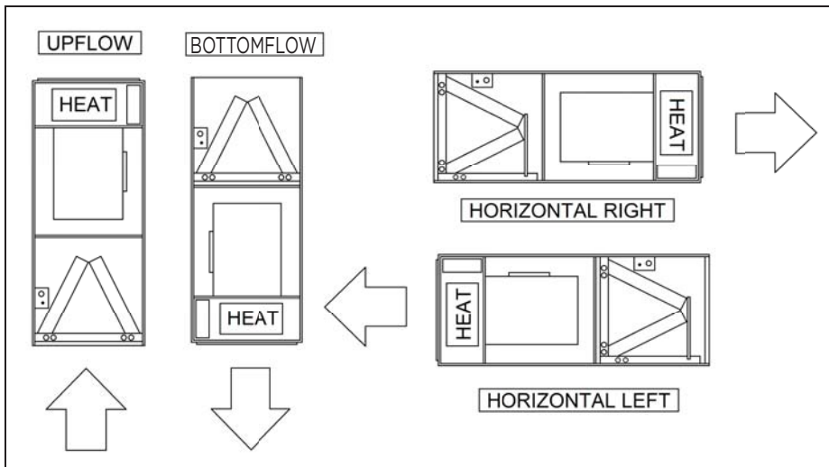
FIGURE 3: Typical Installation Note: Air flow on the O60 and O66 units in the horizontal configuration should be limited to 1900 CFM in cooling mode, or condensate blow off may occur.
